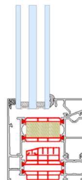
Vast raam Chassis fixe
